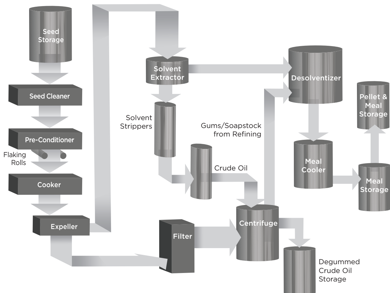
Figure 2. Schematic of solvent extraction process
